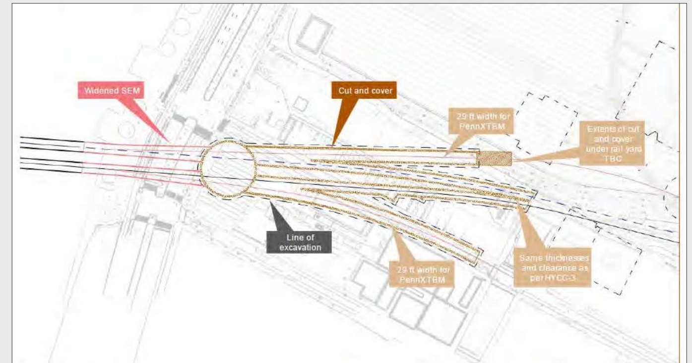
Figure 5-4 Bellmouth Geometry
